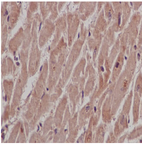
Immunohistochemical analysis of paraffin-embedded human heart, using SHP2 Antibody.
