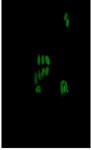
Immunofluorescence analysis of MCF7 cells labelling STAT3 with . The cells were fixed with cold 100% methanol (10min, 4°C) and blocked in 1% BSA/10% normal goat serum/0.3M glycine in 0.1% PBS-Tween 20 for 1h. The cells were then incubated with Goat Anti-Rabbit IgG Fluor488 (1:200, shown in green) at room temperature for 1h
