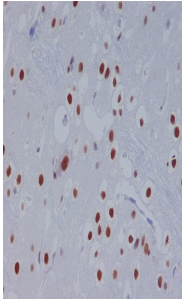
Immunohistochemical analysis of paraffin-embedded rat brain, using STAT3 Antibody.
